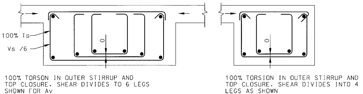
Fig. 12—Recommended two-piece closed single and multiple U-stirrups.
